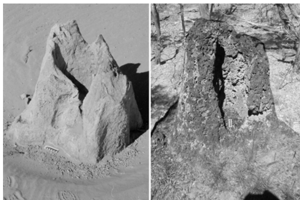
Fig 9: Comparison of a hollow laterite karst pinnacle at White Mountains (right) with a similar limestone pinnacle in syngenetic karst at Nambung, WA (left). Both pinnacles have a central solution pipe and a harder rim and are about 1 m high.
