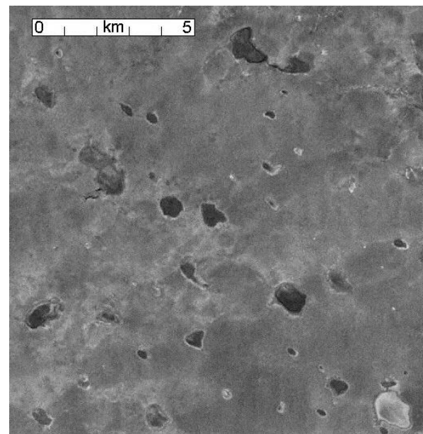
Fig 3: A field of broad but shallow 'pans' (dolines) on a laterite plain in NW Qld (Landsat image).
