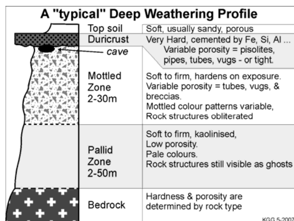
Fig 2: Schematic section through a typical laterite deep weathering profile.
