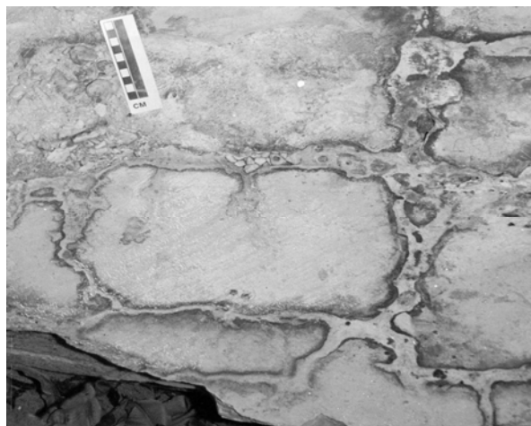
Fig 10: A network of small solution tubelets in a laterite mottled zone of the sea cliffs at Darwin, NT. The tubes have dark ferruginised rims and patches of nodular fill. 10 cm scale-bar.
