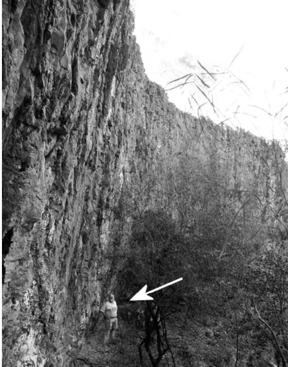
Fig 4: Andy Spate (arrowed) shows the size of this deep collapse doline in a laterite beside the Buchanan Highway, NT.
