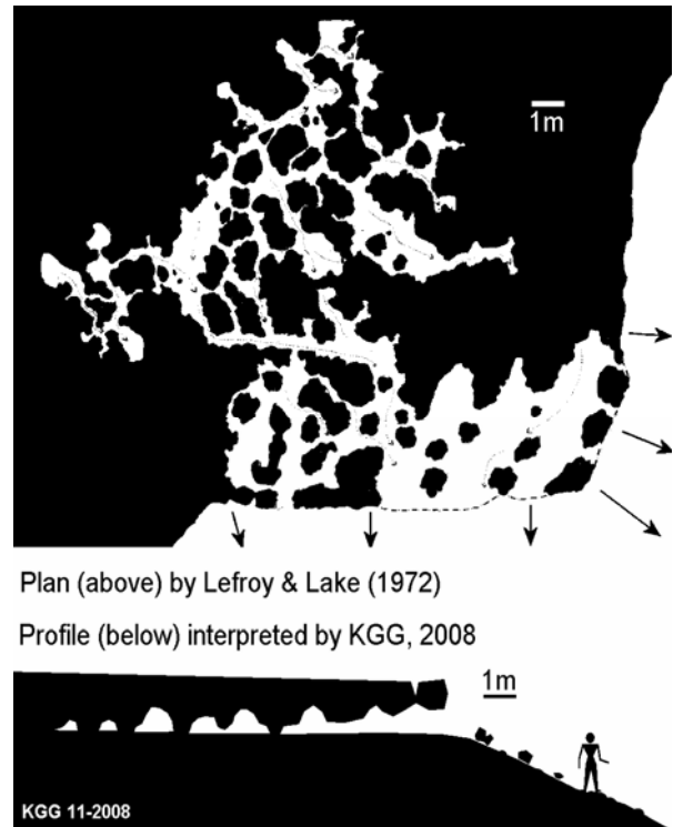
Fig 6: The small laterite maze cave at Chittering, WA. From a map by Lefroy & Lake (1972), a pair of school students who explored and mapped the system as a science project. Ken Grimes has added an interpreted profile. Note the scale bar; many of these passages would be inaccessible to a 'standard-size' adult caver!
